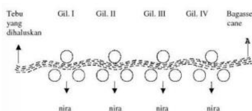
Fig. 8. Sugarcane milling process (Source: [20])
